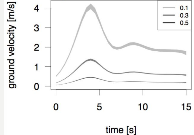
Absolute ground velocity by dynamic coefficient of friction (95% confidence intervals)
