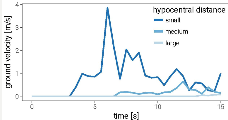
Typical observations by hypocentral distance
